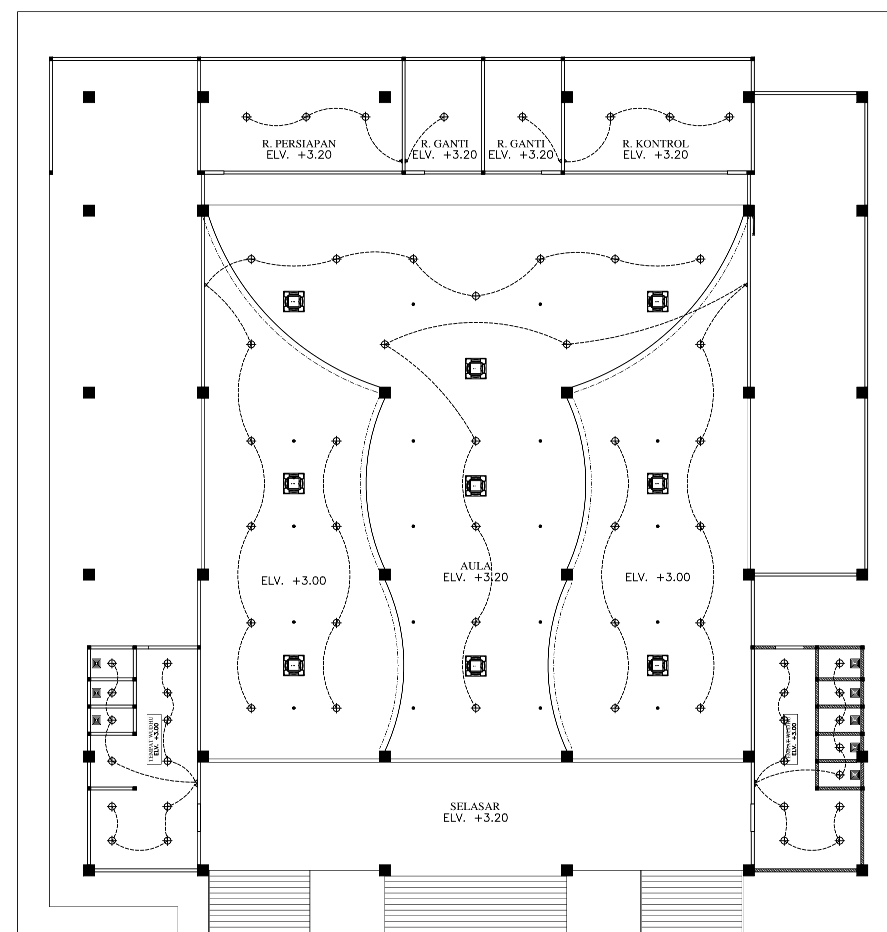
DENAH CEILING LANTAI DASAR (AULA) SCALE 1 : 450
