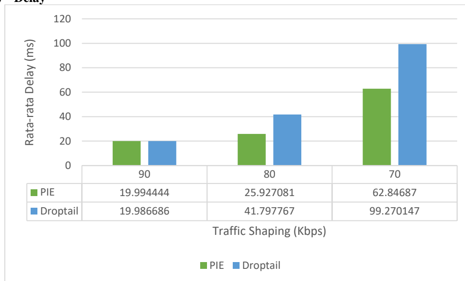
Gambar 3- Rata-rata Delay PIE dan,Droptail
