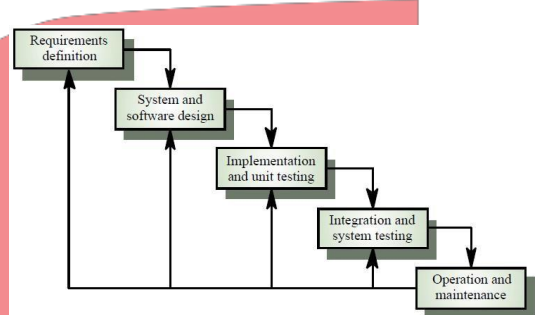
Gambar 1 - 1 Metode Waterfall [1]
