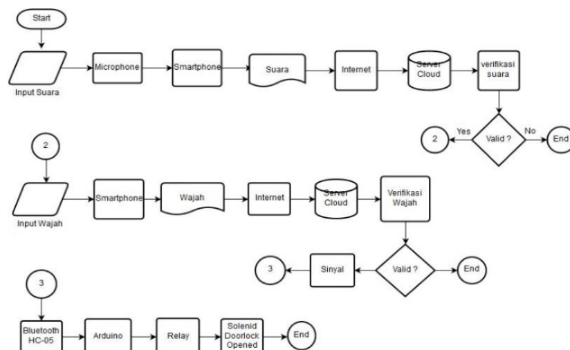
Gambar 2 Flowchart Sistem
