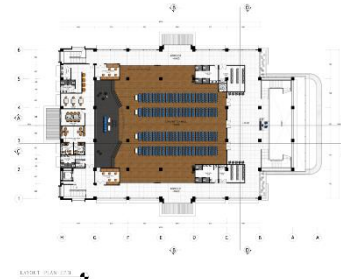
Gambar 6. Layout Lt 3
