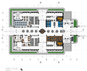
Gambar 4. Layout Lt 1
