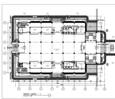
Gambar 2. Denah Eksisting Lt 1
