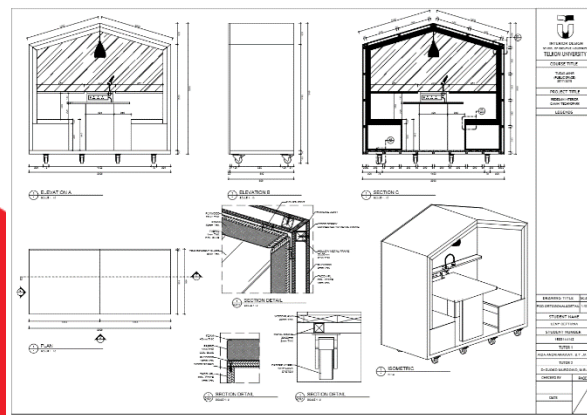
Gambar 11. Desain furniture
