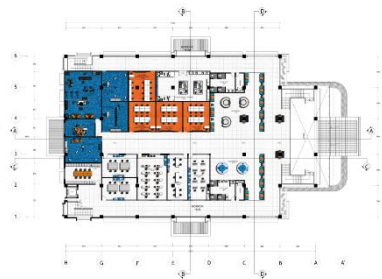
Gambar 5. Layout Lt 2
