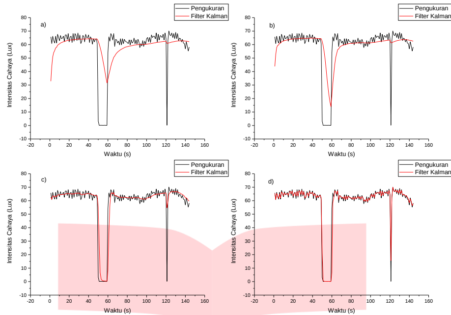
Gambar 4. 6 a) Measurement Noise Covariance = 2 b) Measurement Noise Covariance = 1 c) Measurement Noise Covariance = 0.1 d) Measurement Noise Covariance = 0.01
