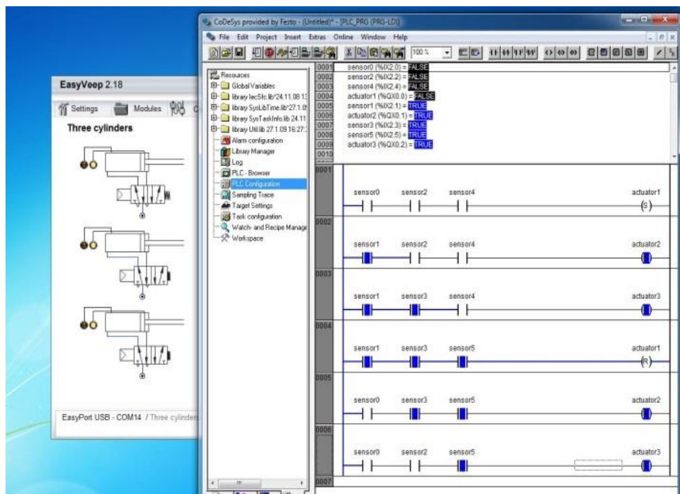
Gambar 2.1 Ladder programming
