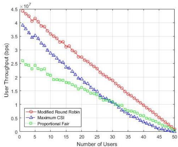
Figure 6. User Throughput
