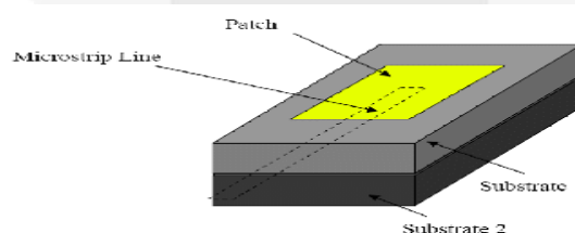
Gambar 2. Proximity Coupled
