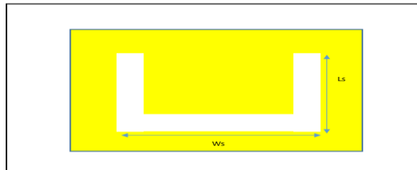
Gambar 3. U-Slot
