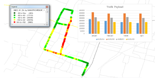
Gambar 3 Drivetest_RSCP_Download
