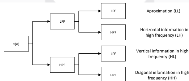
Gambar 2.1 Diagram SWT filter bank 2 level [6]
