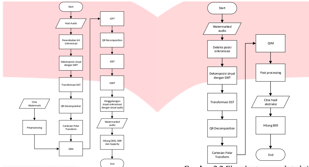
Gambar 3.1 Flowchart proses embedding
