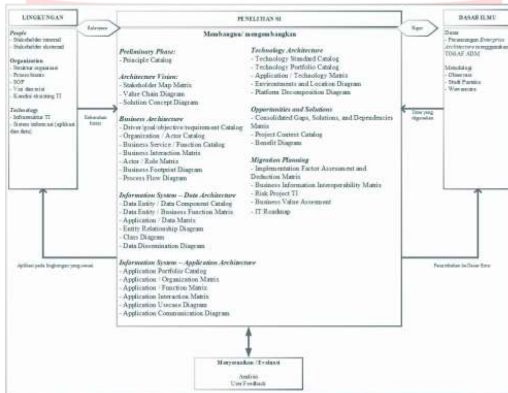
Gambar 1 Model Konseptual
