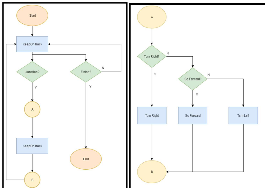
Gambar 3.2 Diagram Alir
