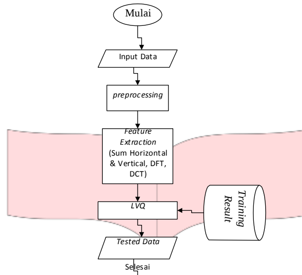
Gambar 4 Flowchart Tested Data[8]
