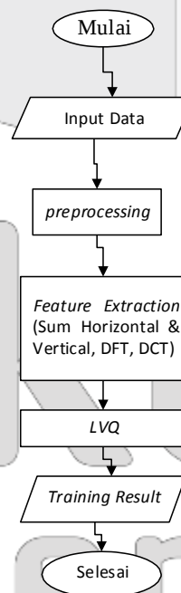
Gambar 3 Flowchart Training Data[8]
