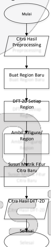
Gambar 10 Diagram Alir DFT-2D[11]
