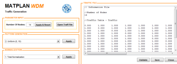
Fig. 3. Generating Traffic
