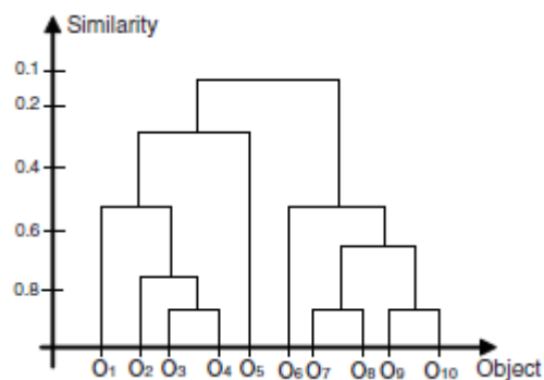
Gambar I.1 Contoh Dendrogram
