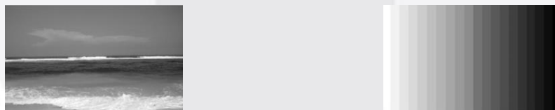
Gambar 2.15 Citra grayscale
