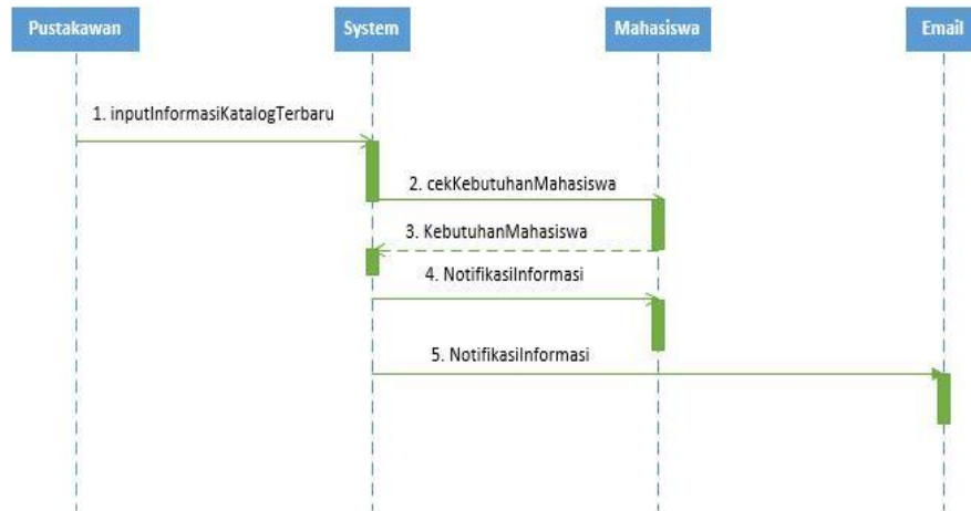
Gambar 4. 1 Sequence Update Informasi
