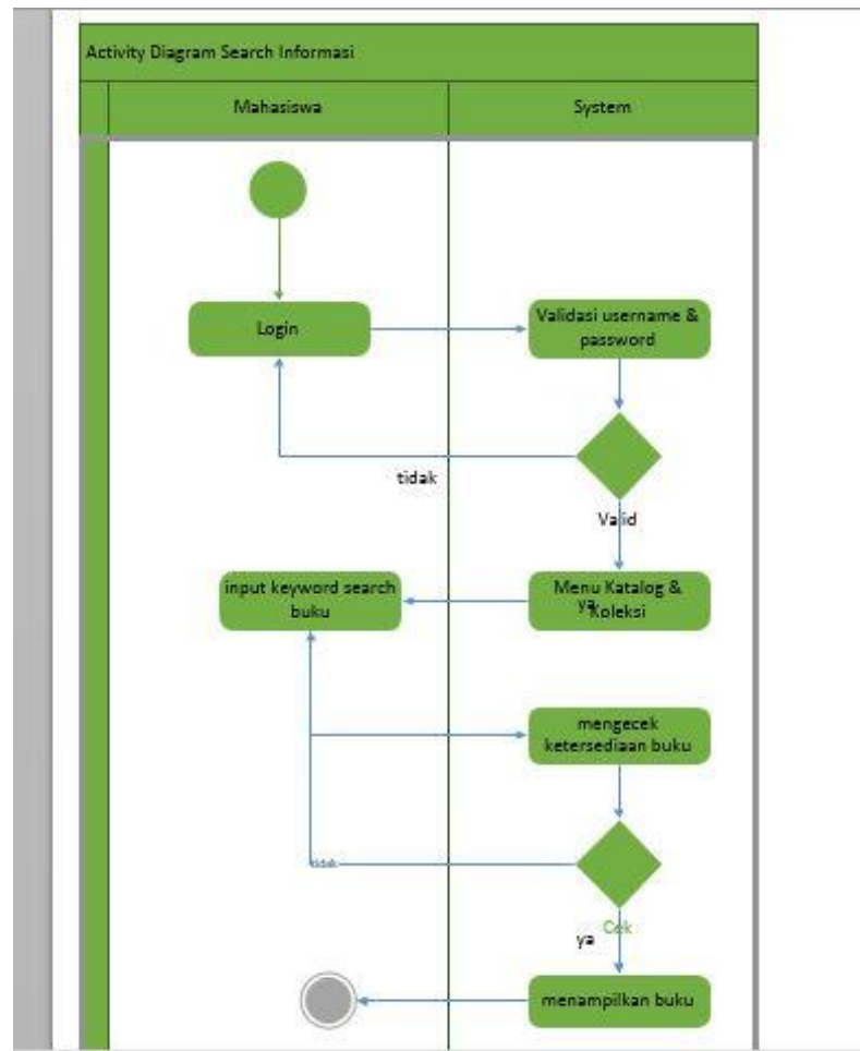
Gambar 4. 2 Activity Diagram Pencarian Buku
