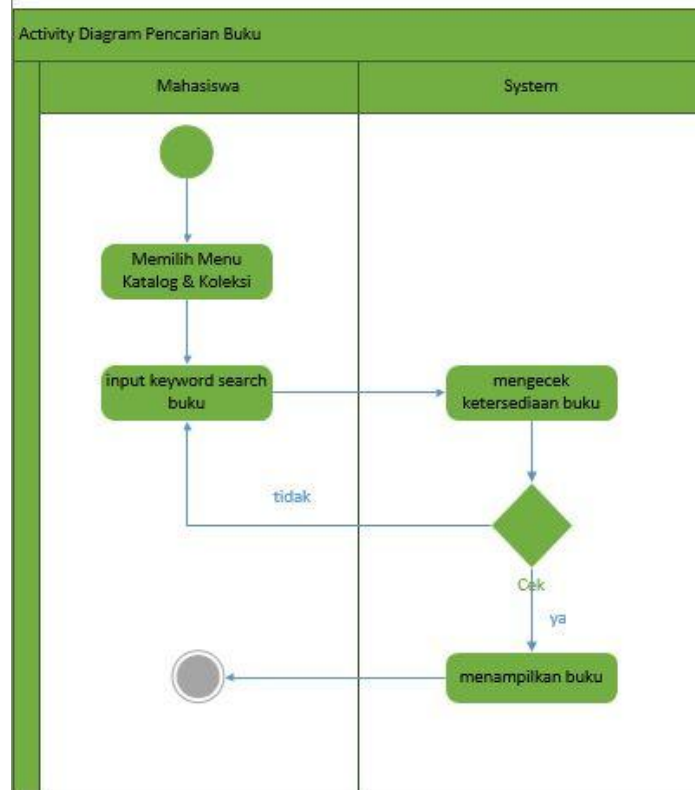
Gambar 4. 4 Activity Diagram Completeness
