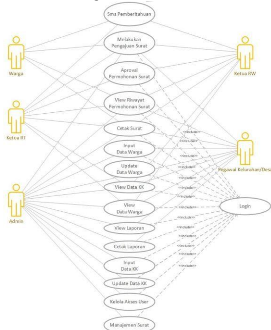
Gambar 5. Usecase diagram
