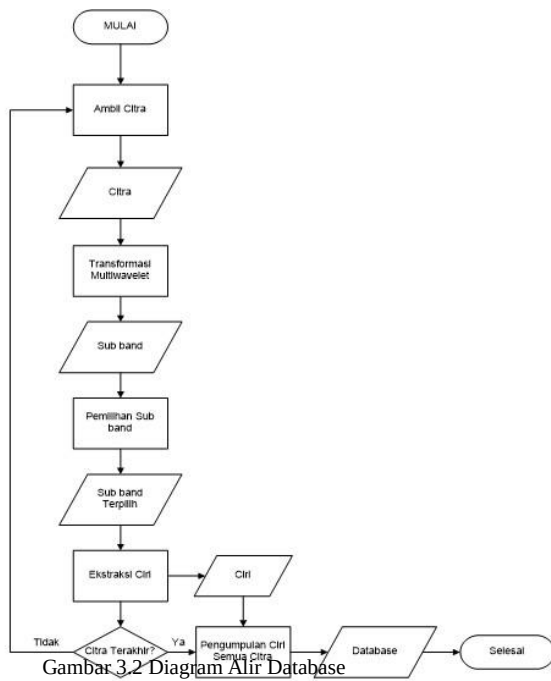
Gambar 3.2 Diagram Alir Database
