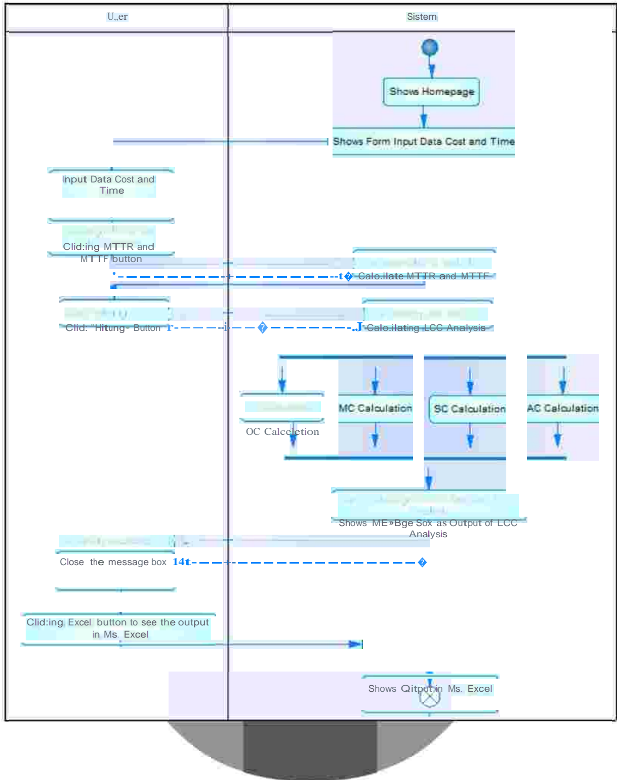
Figure 3.2 Activity Diagram
