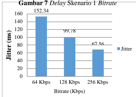
Gambar 7 Delay Skenario 1 Bitrate
