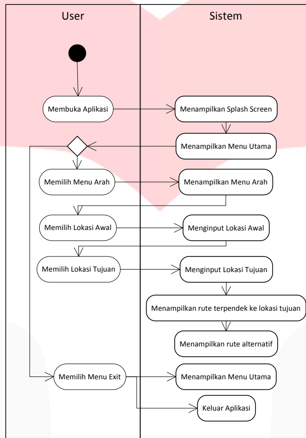
Gambar 4.3 Activity Diagram
