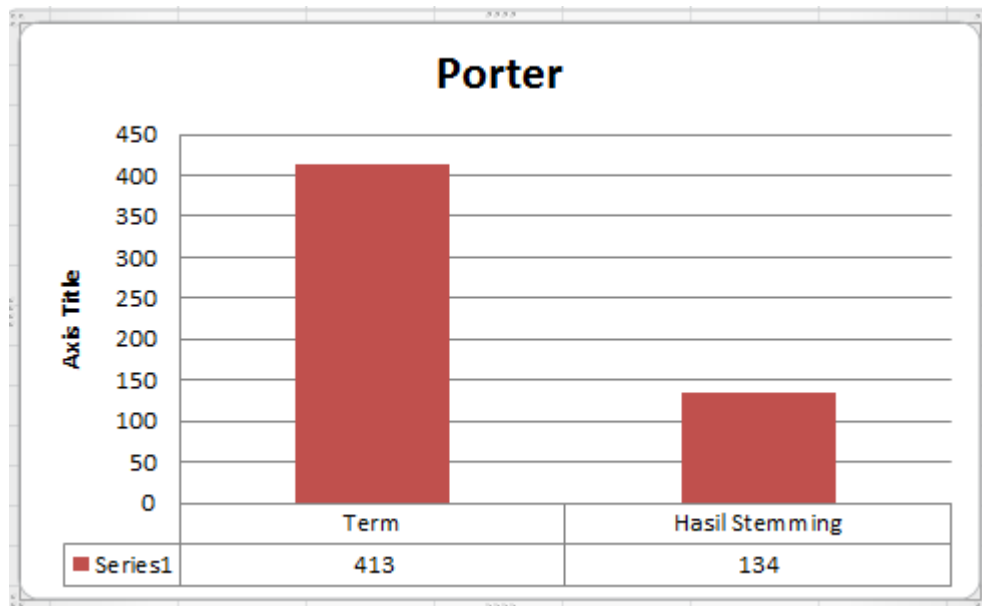
Gambar 3.2 Hasil stemming Porter
