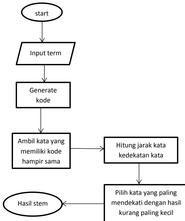
Gambar 3.0.1 Alur proses stemming
