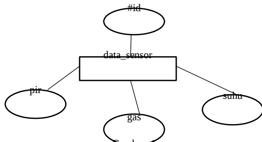
Gambar 1 ER-Diagram data_sensor
