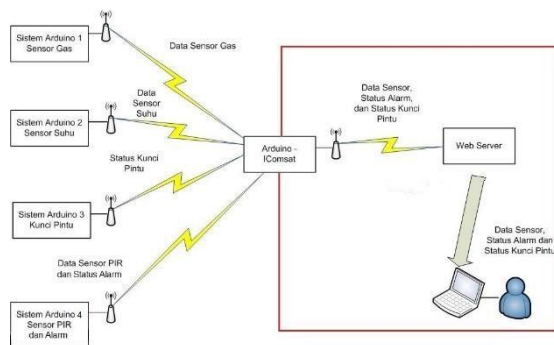
Gambar 3 Blok Diagram Sistem Web User Interface
