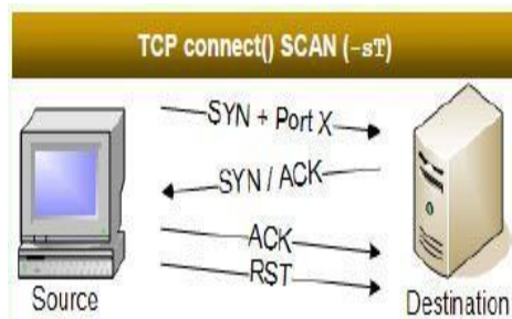
Gambar 2-3 TCP Scanning
