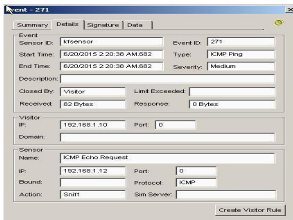
Gambar 4-11 Serangan Ping
