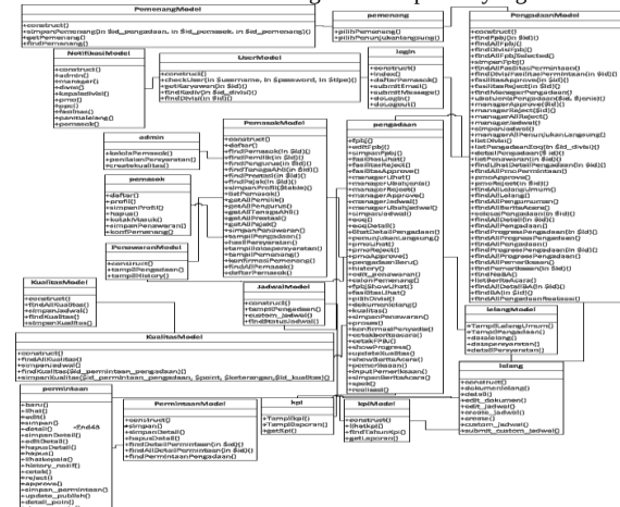
Gambar 3 Class Diagram
