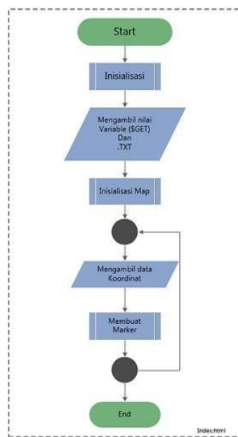
Gambar 10: Flowchart index.html
