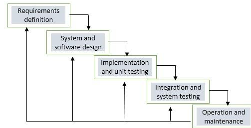
Gambar 1 Model Waterfall
