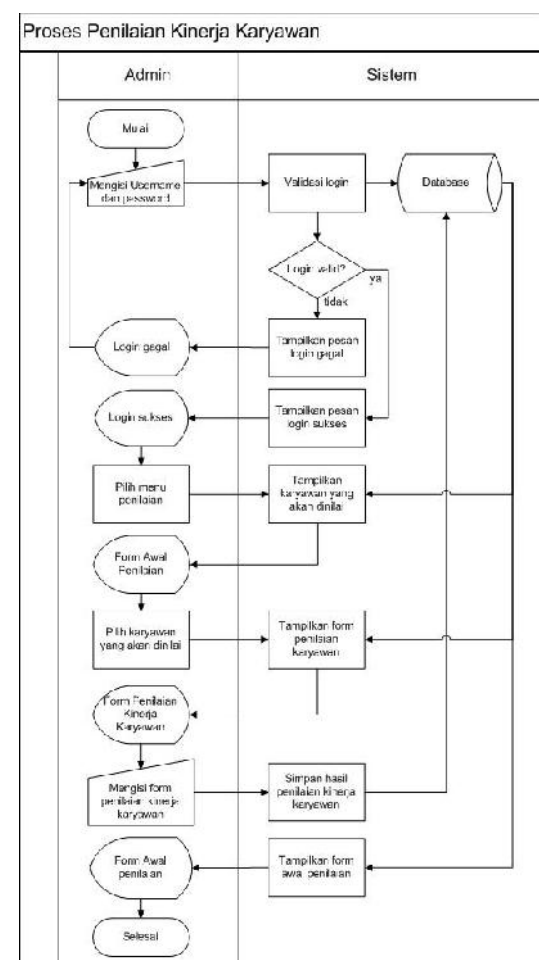
Gambar 3. 1 Flowmap usulan proses penilaian kinerja karyawan
