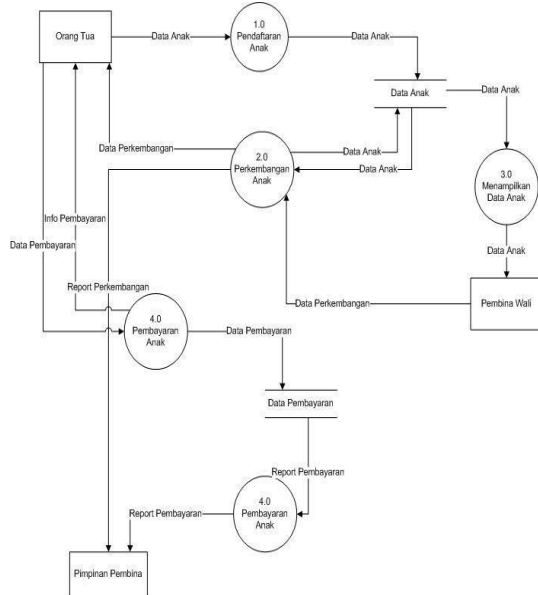
Gambar 3 DFD Level 1
