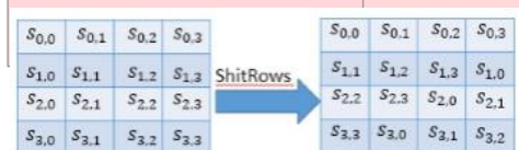
Gambar 2.4.4 Proses ShiftRows [3]
