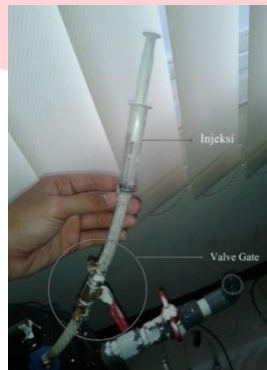
Gambar 4 Sistem injeksi larutan \text{CaCO}_3 .
