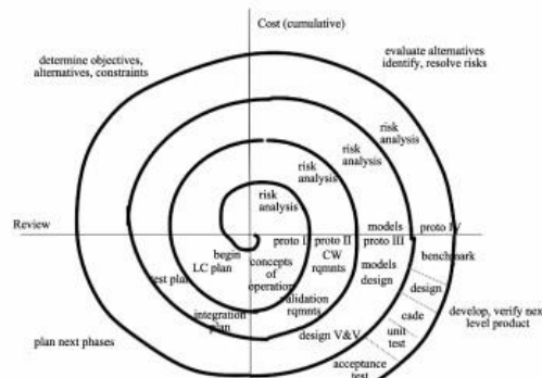
Gambar 2 Model Spiral [6]
