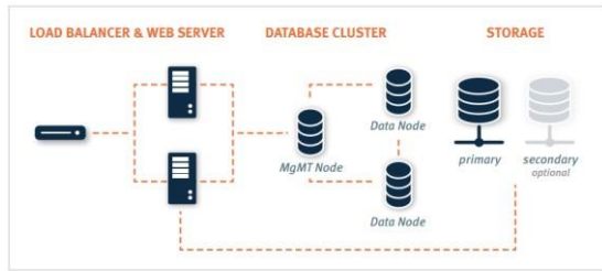
Gambar 5 Arsitektur Deployment Owncloud [6]
