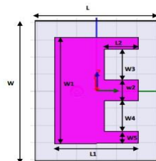
Gambar 2.1 Struktur antenna E-shaped
