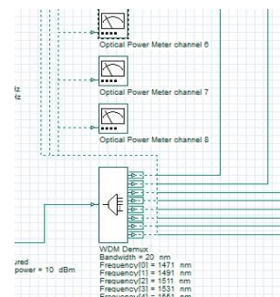
Gambar 10, Optical power meter
