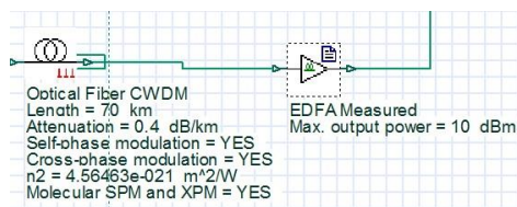
Gambar 8, EDFA
