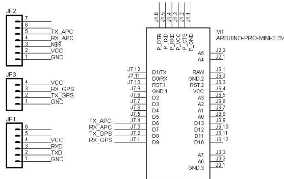
Gambar 9: Desain Schematic
