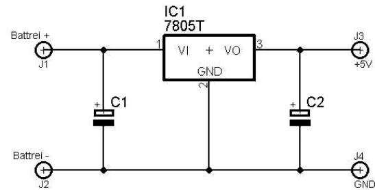
Gambar 11: Schematic Regulator
