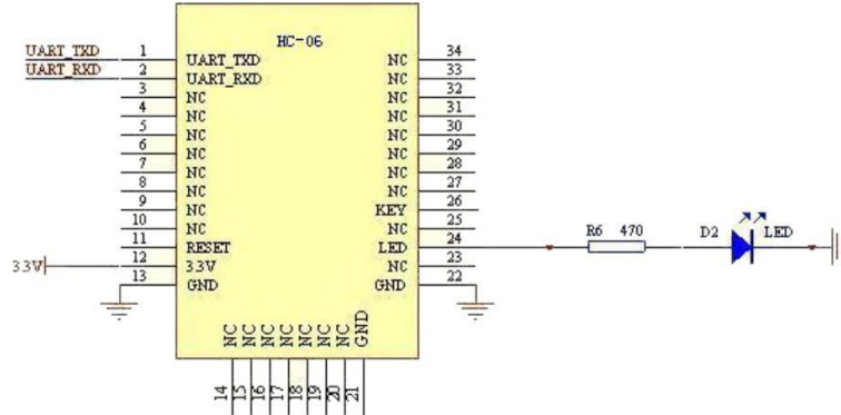
Gambar 3.5 Shield Bluetooth
