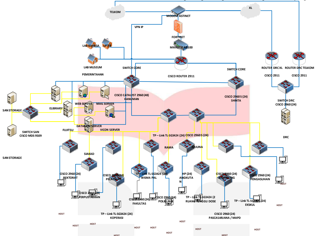
Gambar 5 Communications Engineering Diagram Institut XYZ
