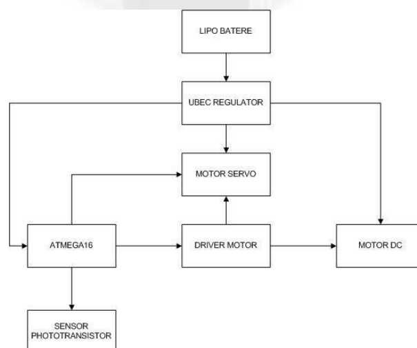
Gambar 1 Blok Diagram
