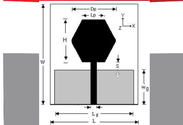
Gambar 1 Antena Mikrostrip Patch Hexagonal [10]
