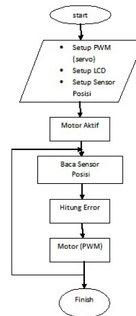
Gambar 3.7 Flowchart sistem horizontal
