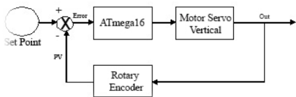
Gambar 3.1 Blok Diagram Vertical
