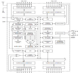
Gambar 2.7 Blok Diagram ATmega16
