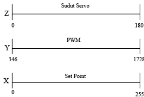
Gambar 3.5 Interpolasi Set Point,PWM, dan Sudut Servo
