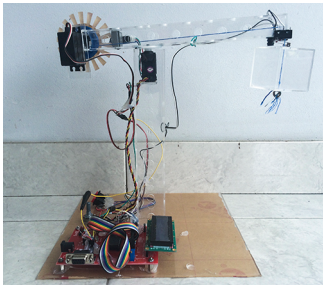
Gambar 3.1 Model Sistem
