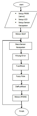
Gambar 3.6 Flowchart sistem vertical
