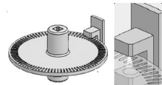
Gambar 2. 12 Rotary Encoder
