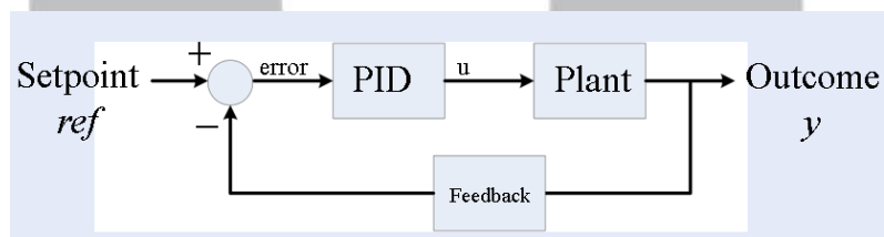
Gambar 5. Diagram Blok PID
