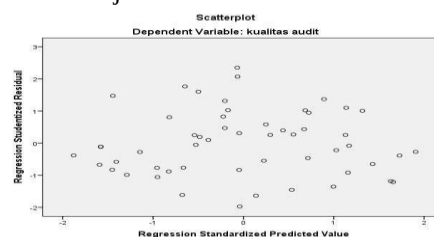
Gambar 1. Scatterplot
