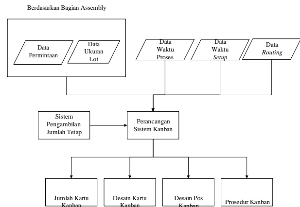
Gambar III.1 Metodologi Penelitian
