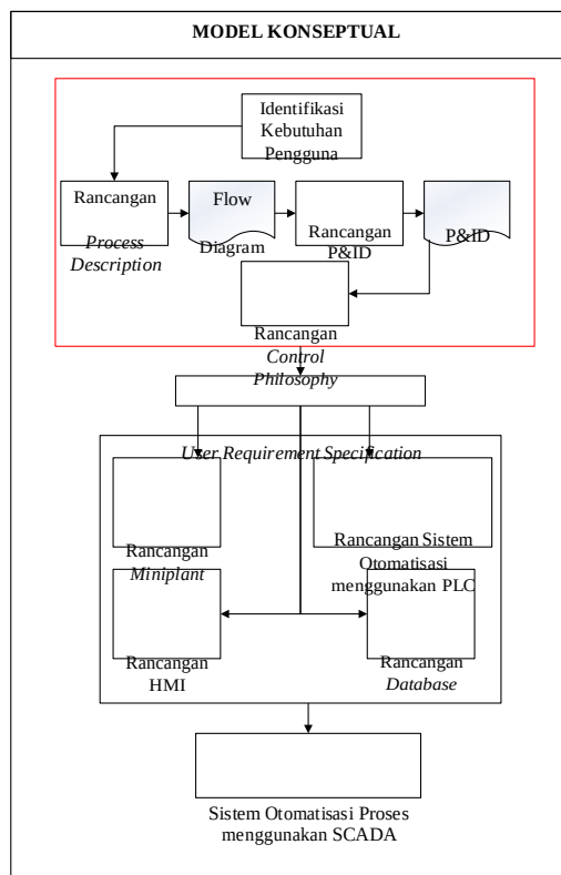
Gambar III. 1 Model Konseptual
