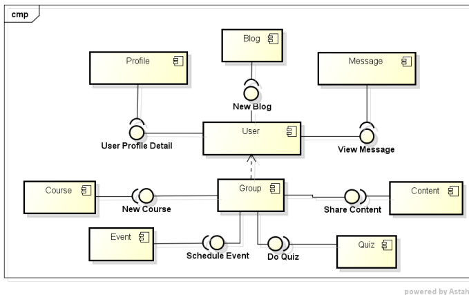
Gambar 13 Component Diagram Social e-Learning
