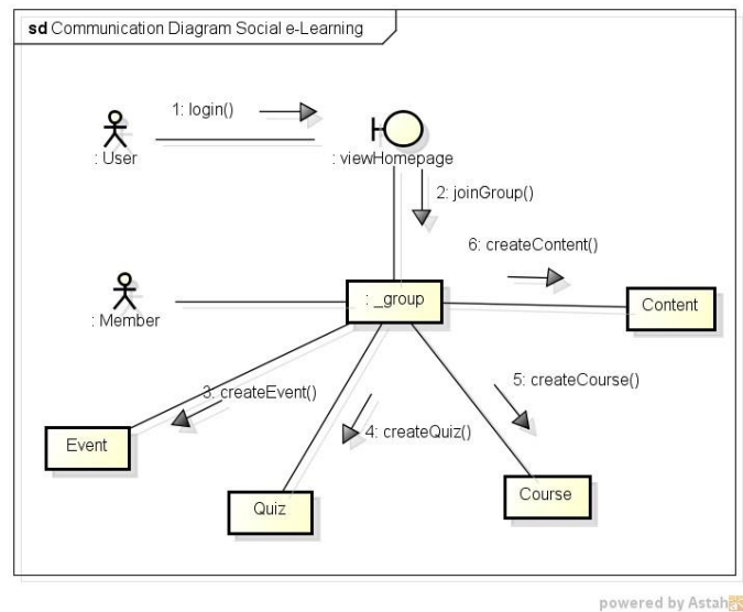
Gambar 9 Communication Diagram Social e-Learning
