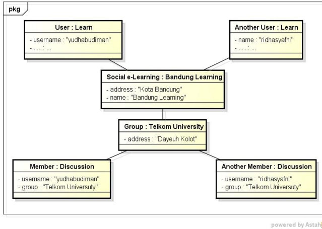
Gambar 11 Object Diagram Social e-Learning
