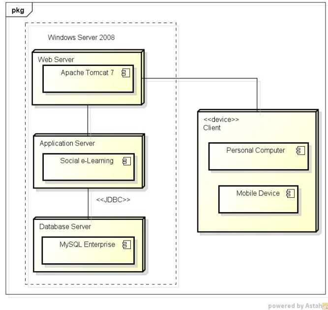
Gambar 14 Deployment Diagram Social e-Learning
