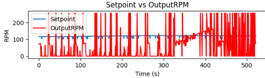
Figure 4. 14 Graph of Setpoint vs. OutputRPM in Adaptive PID
