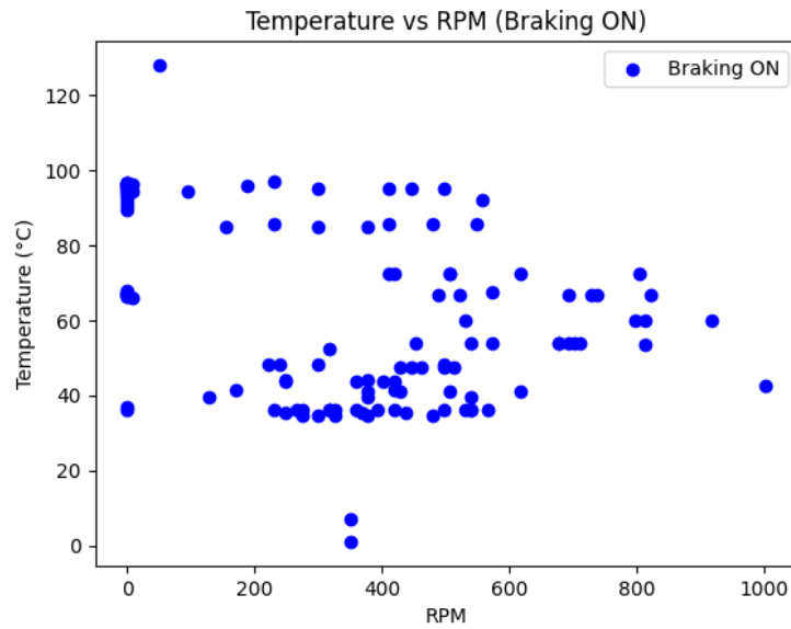
Figure 4. 7 Scatter Plot of Regenerative Braking with No Control
