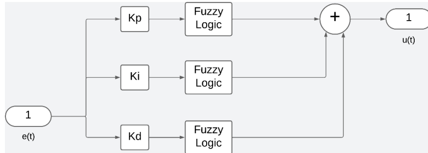
Figure 2. 8 Hybrid PID-Fuzzy based control [22]
