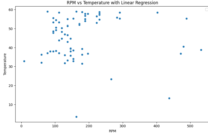
Figure 4. 22 Scatter Plot of Regenerative Braking with Hybrid Fuzzy-PID 2
