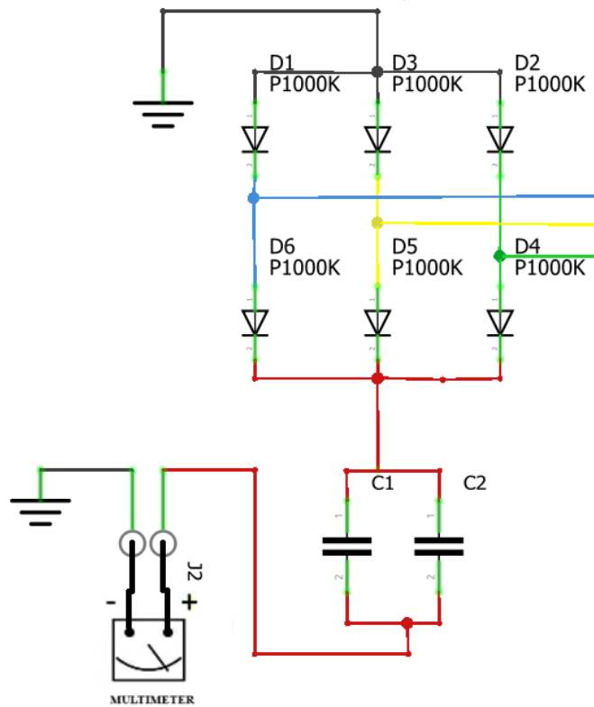
Figure 4. 1 Schematic of Voltage Output Check for Regenerative Braking System
