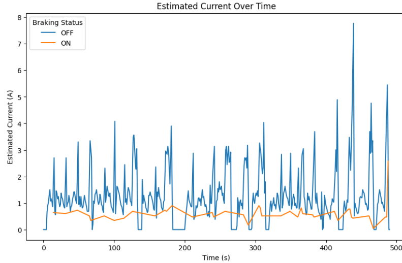
Figure 4. 17 Graph of Estimated Current vs. Regenerative Braking Time with Hybrid Fuzzy-PID 1
