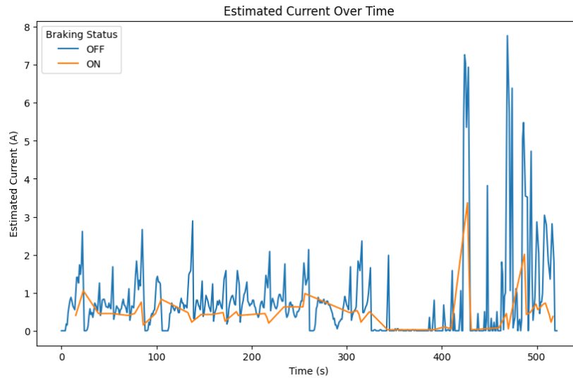
Figure 4.13 Graph of Estimated Current vs. Regenerative Braking Time with Adaptive PID
