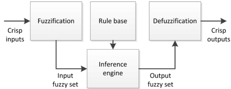
Figure 2. 6 Fuzzy Logic Control Block Diagram
