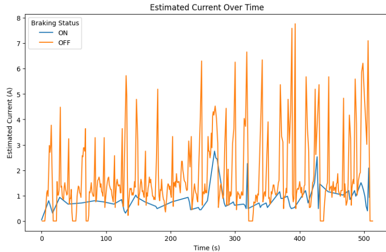
Figure 4.19 Graph of Estimated Current vs. Regenerative Braking with Hybrid Fuzzy-PID 2
