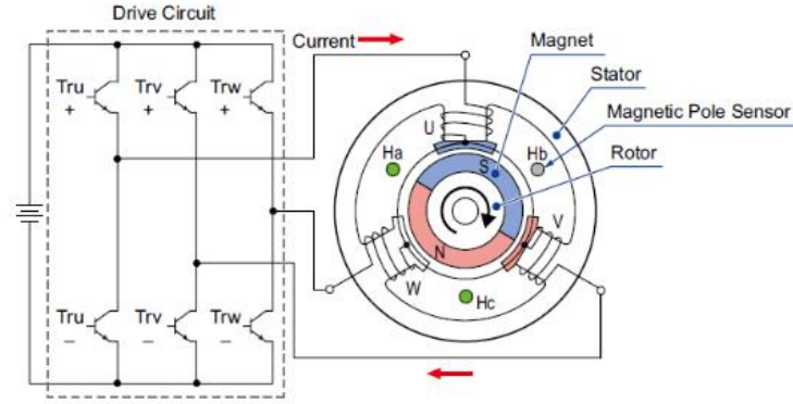
Figure 2. 2 BLDC Motor's Diagram
