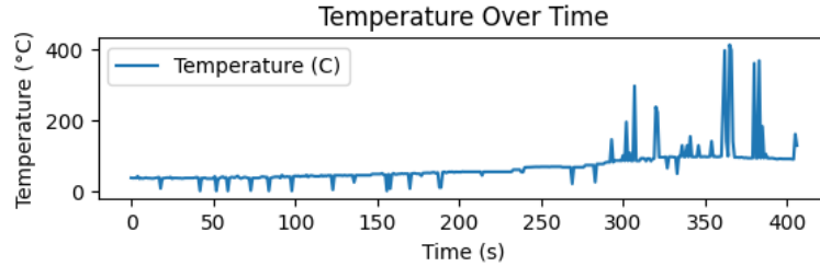
Figure 4. 5 Graph of Temperature vs. Regenerative Braking Time with No Control
