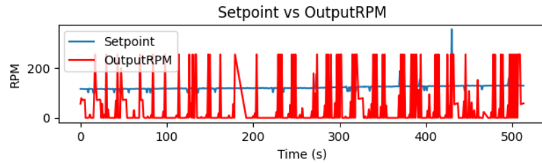
Figure 4. 20 Graph of Setpoint vs. OutputRPM in Hybrid Fuzzy-PID 2
