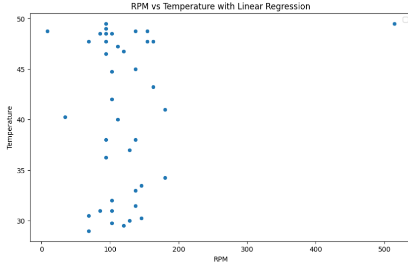
Figure 4. 21 Scatter Plot of Regenerative Braking with Hybrid Fuzzy-PID 1
