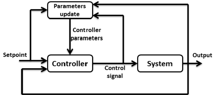
Figure 2. 7 Adaptive PID Control Block Diagram
