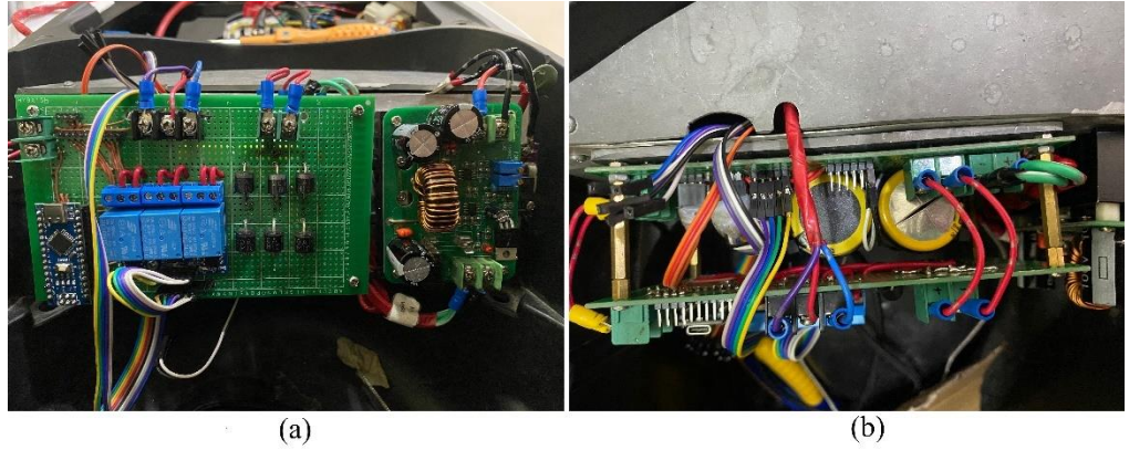
Figure 3. 7 Regenerative Braking System Controller: (a) Top view, (b) Side view
