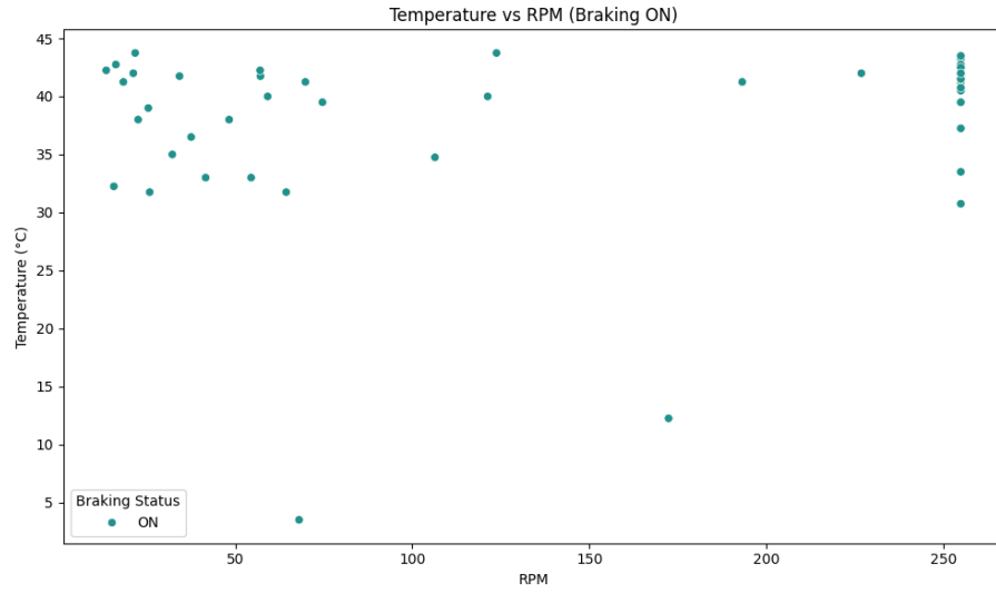
Figure 4. 15 Scatter Plot of Regenerative Braking with Adaptive PID
