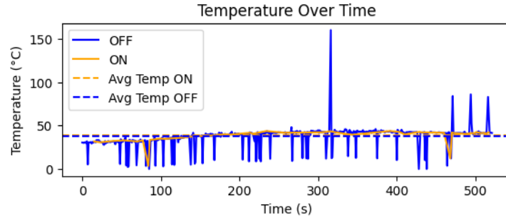
Figure 4.12 Graph of Temperature vs. Regenerative Braking Time with Adaptive PID
