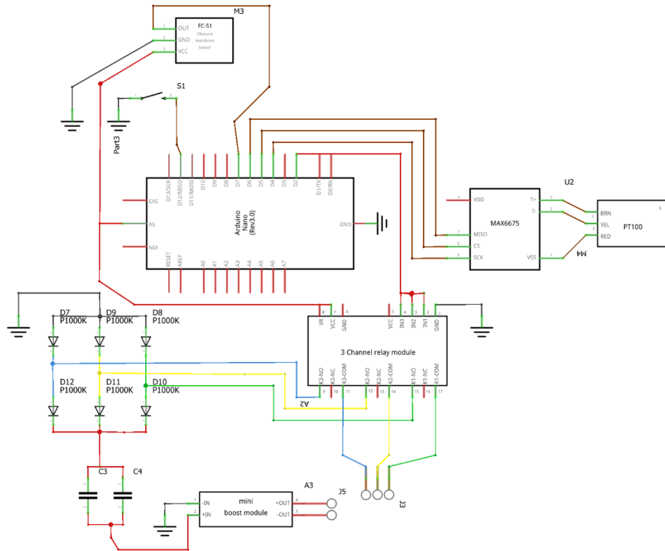
Figure 3. 4 Regenerative Braking System Schematic
