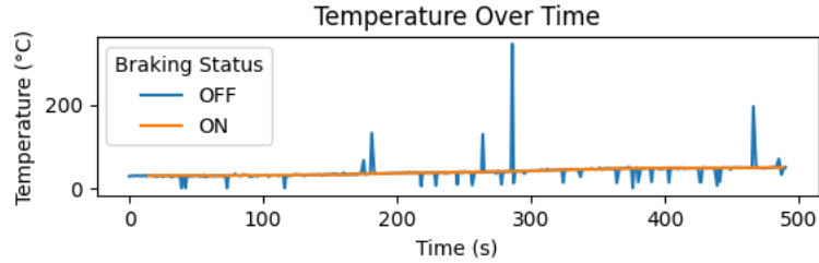
Figure 4. 16 Graph of Temperature vs. Regenerative Braking Time with Hybrid Fuzzy-PID 1
