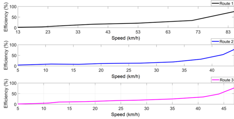
Figure 2.4 Regenerative Braking Efficiency at a Specific Speed[16]
