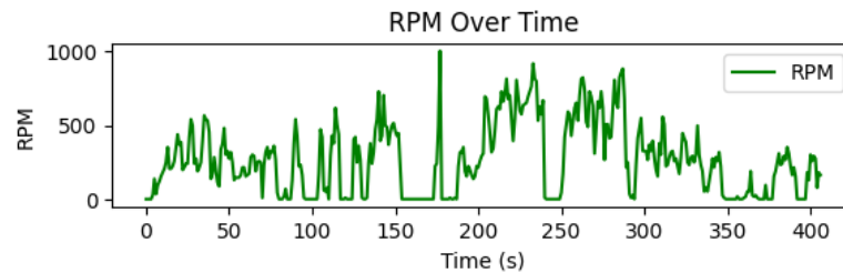
Figure 4. 6 Graph of RPM vs. Regenerative Braking Time with No Control
