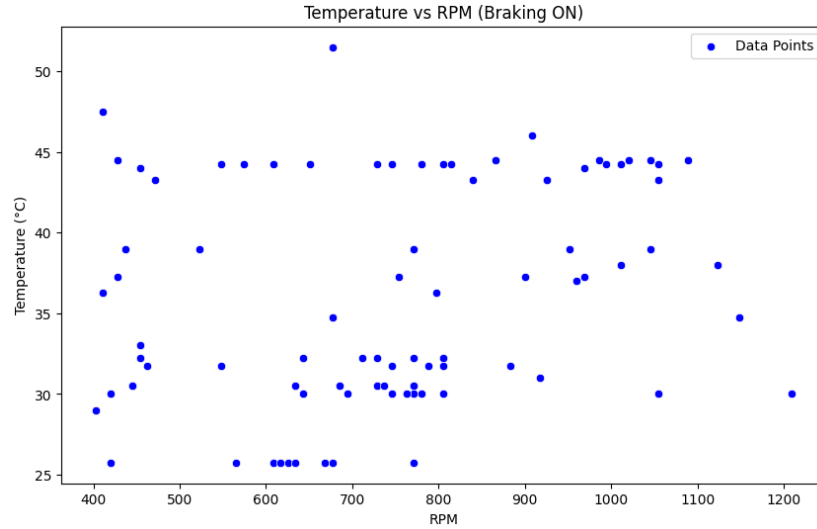
Figure 4. 11 Scatter Plot of Regenerative Braking with Fuzzy Logic
