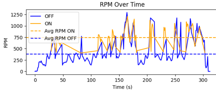
Figure 4. 9 Graph of RPM vs. Regenerative Braking Time with Fuzzy Logic
