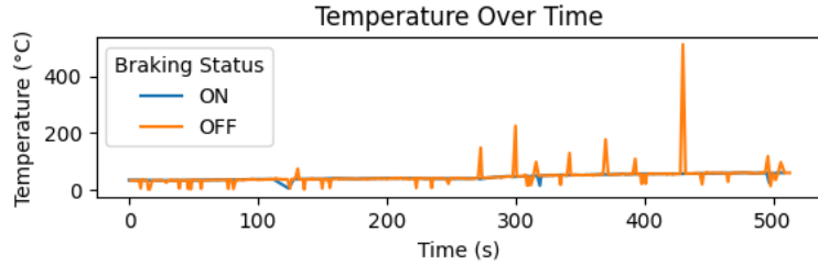
Figure 4.18 Graph of Temperature vs. Regenerative Braking Time with Hybrid Fuzzy-PID 2
