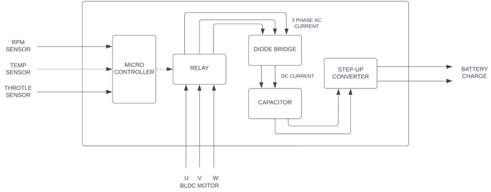
Figure 3. 5 Regenerative Braking System Function Block Diagram
