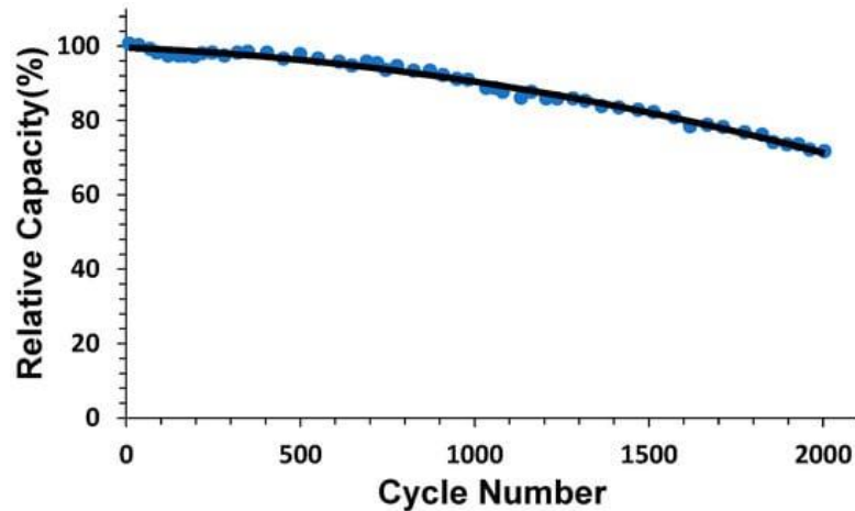
Figure 2. 5 graph of Relative Capacitance vs. Number of Cycles for Kokam SLBP5520510H Battery [18]
