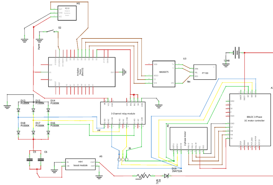
Figure 3. 2 System's Schematic
