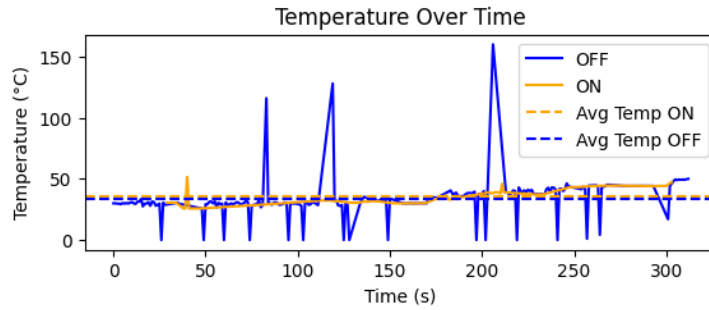
Figure 4. 8 Graph of Temperature vs. Regenerative Braking Time with Fuzzy Logic
