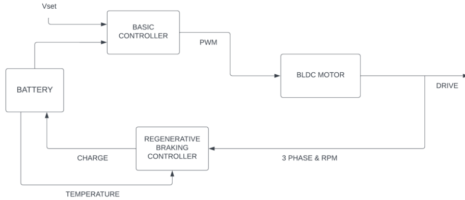
Figure 3. 1 System's Block Diagram
