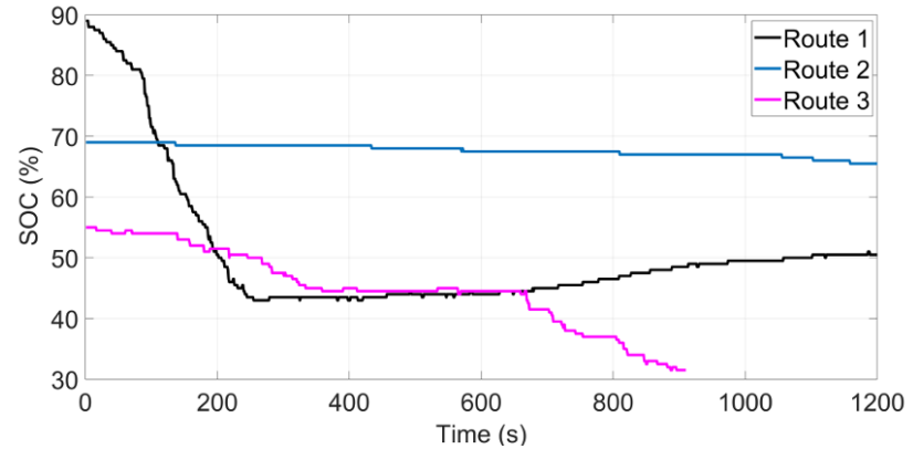
Figure 2. 3 SoC Behavior Related to Recovered Energy [16]
