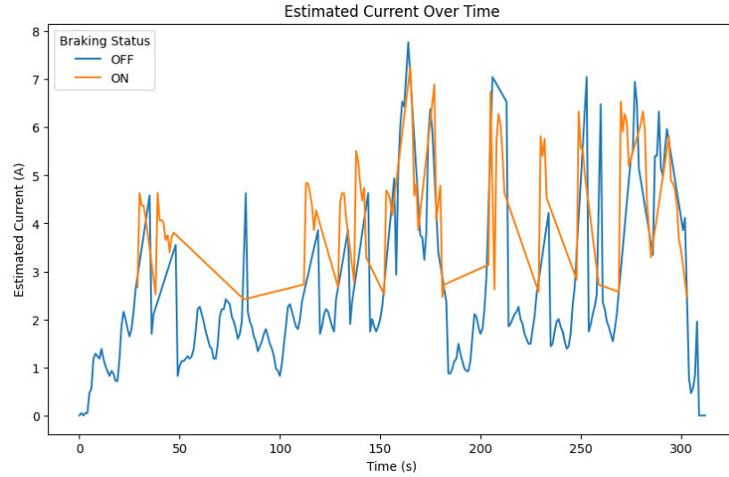
Figure 4. 10 Graph of Estimated Current vs. Regenerative Braking Time with Fuzzy Logic
