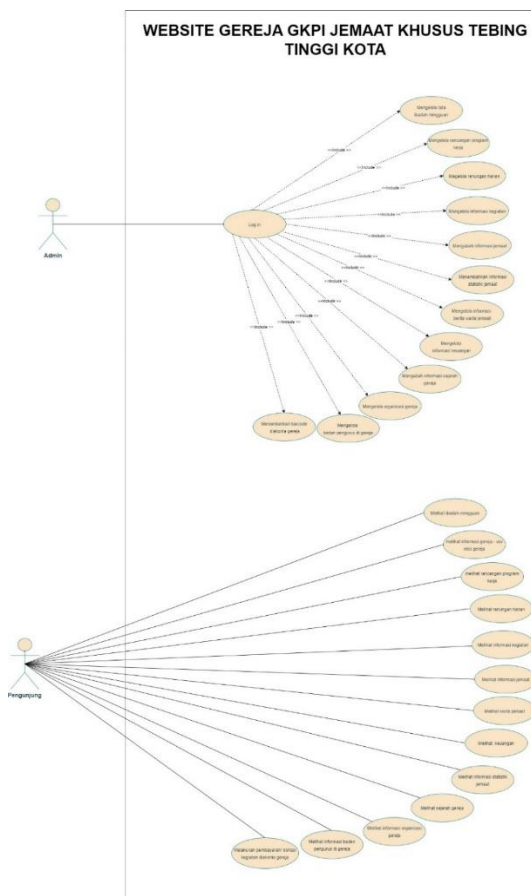
Gambar 4.1 – Use Case Diagram
